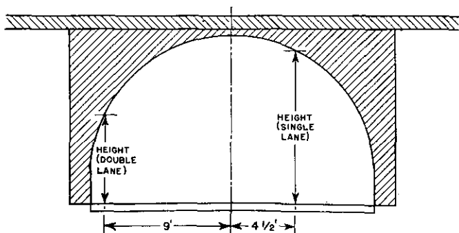
FIGURE 9.—Standard method of measuring vertical clearances under arches.
