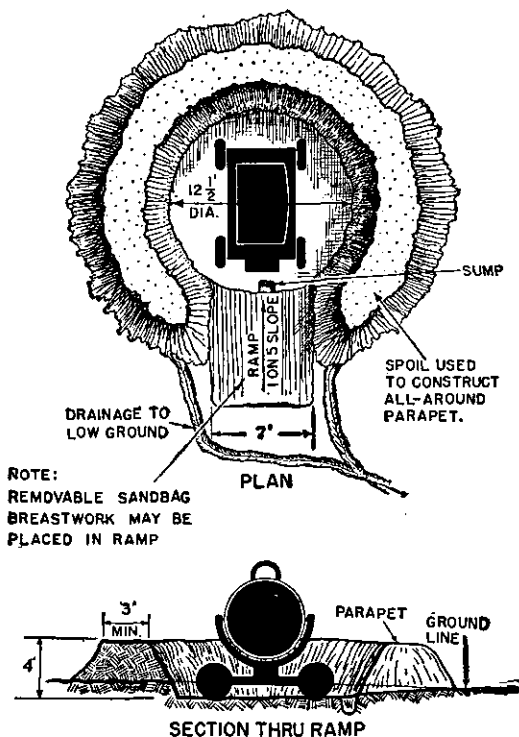
Figure 63. Searchlight emplacement. (Camouflage omitted.)
