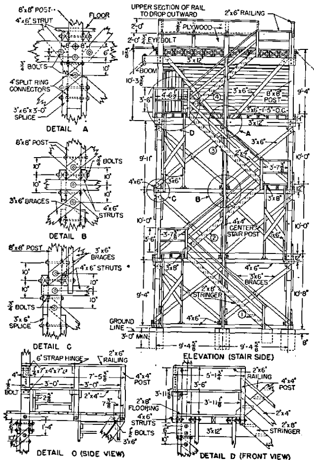
② Elevation stair, side and details.
