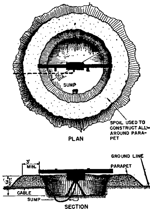
Figure 57. Emplacement for height finder M1 or M2. (Camouflage omitted.)
