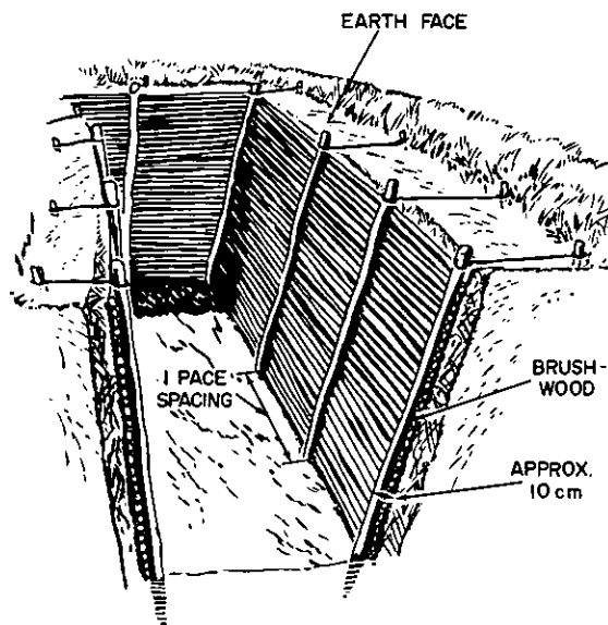
Figure 4-19. Continuous brush revetment.
