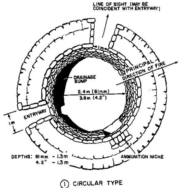
Figure 2-22. Mortar emplacements.
