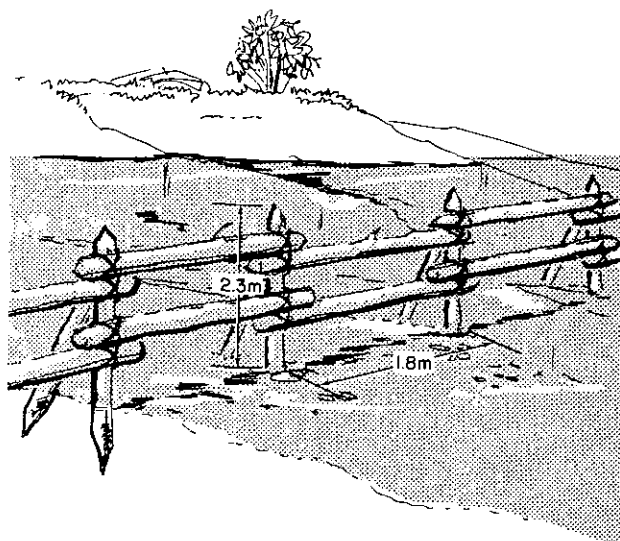
Figure 8-4. Log scaffolding.
