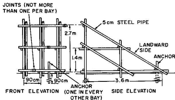
Figure 8-9. Steel scaffolding.
