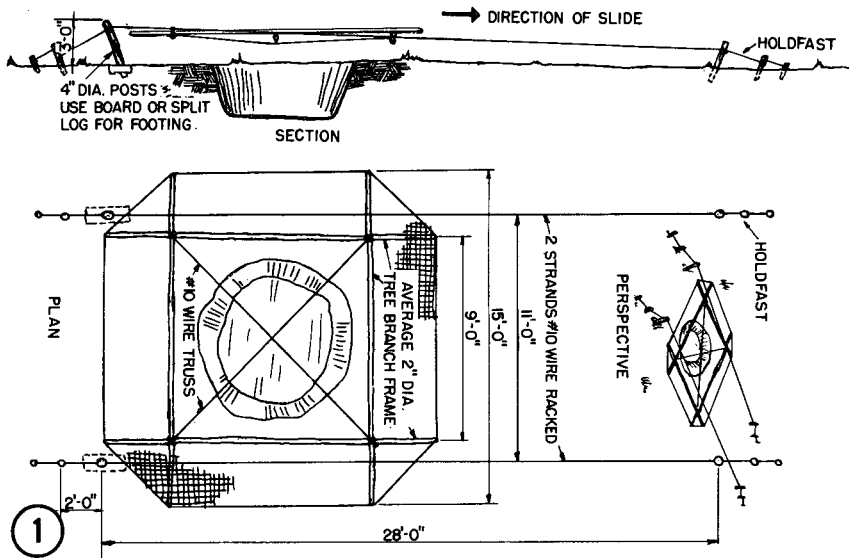
1 Sliding cover construction
