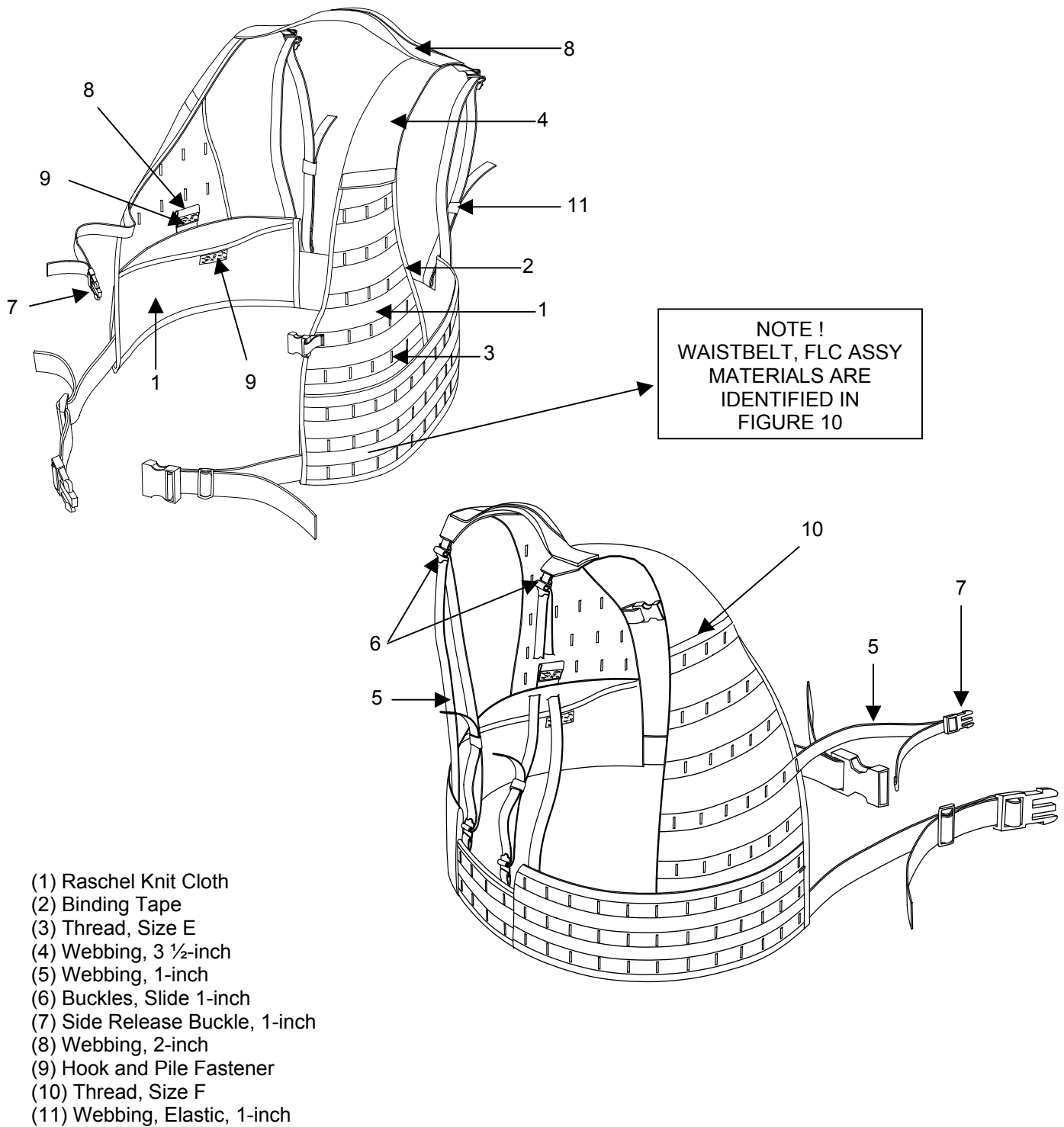
Figure 27-2. Vest, Fighting Load Carrier
