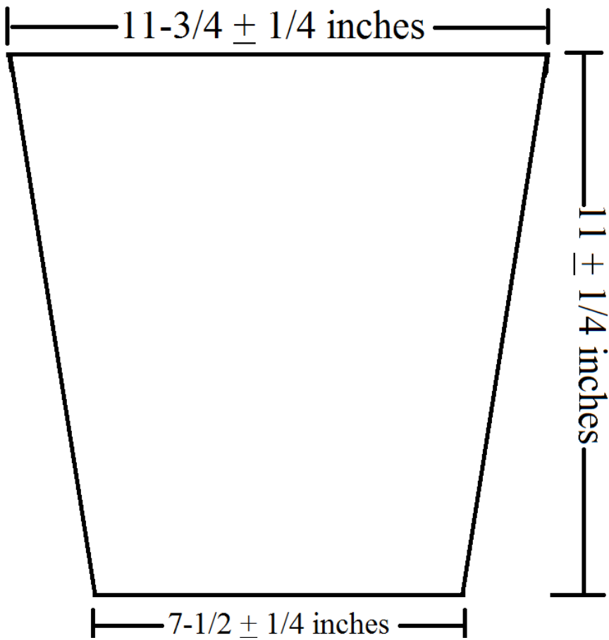
FIGURE 5. Test Specimen, % Bite Protection Test
