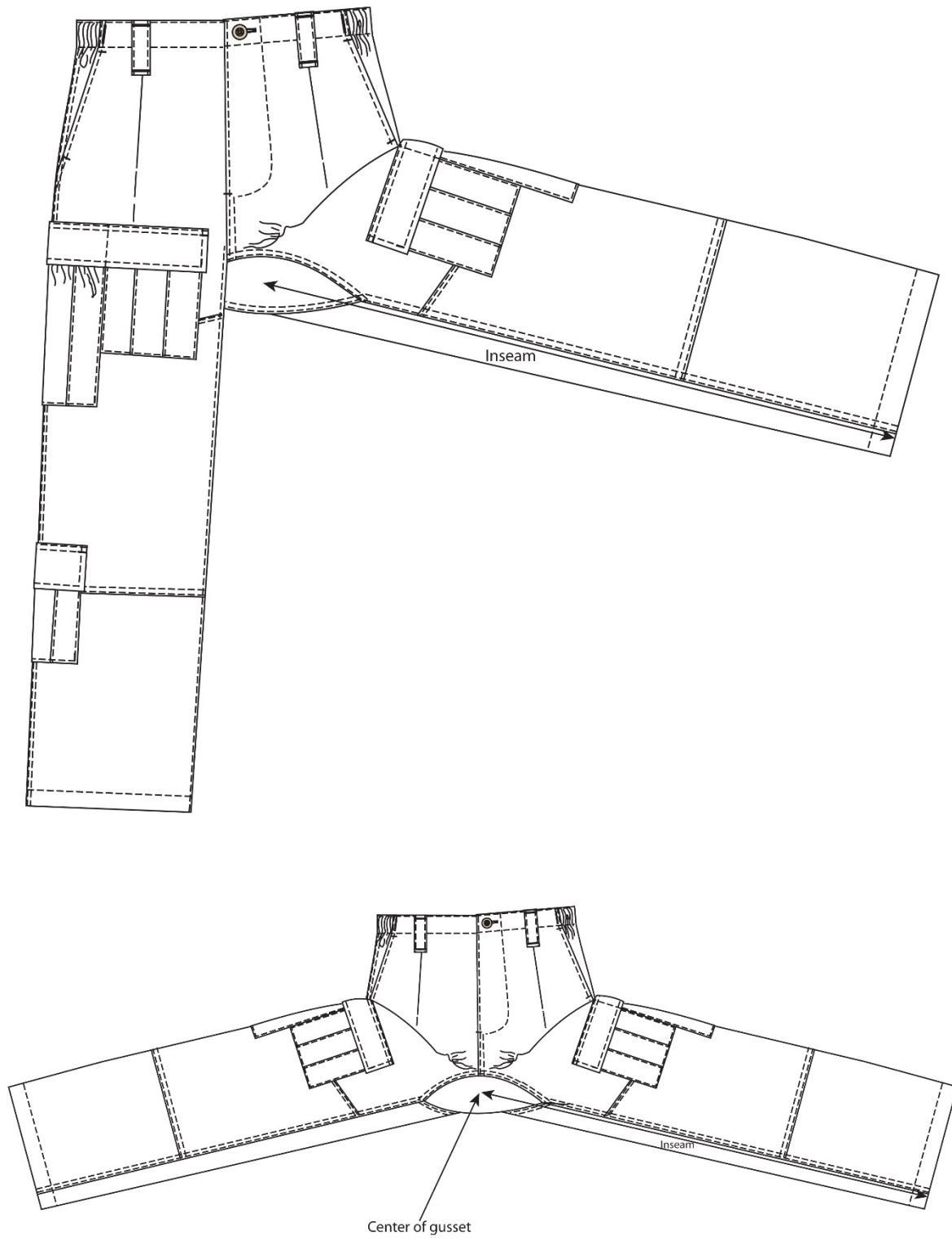
Figure 13. Trouser Inseam Finished Dimension
