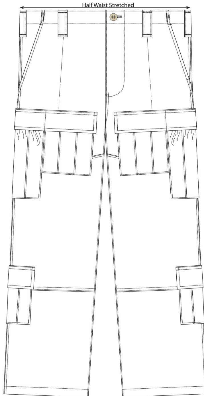
Figure 12. Half Waist Stretched Finished Dimension
