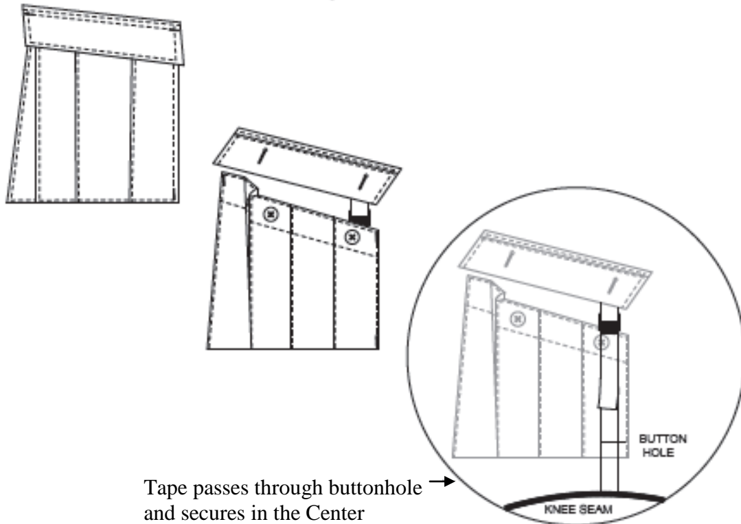
FIGURE 4. Pant, Army Combat, cargo pocket
