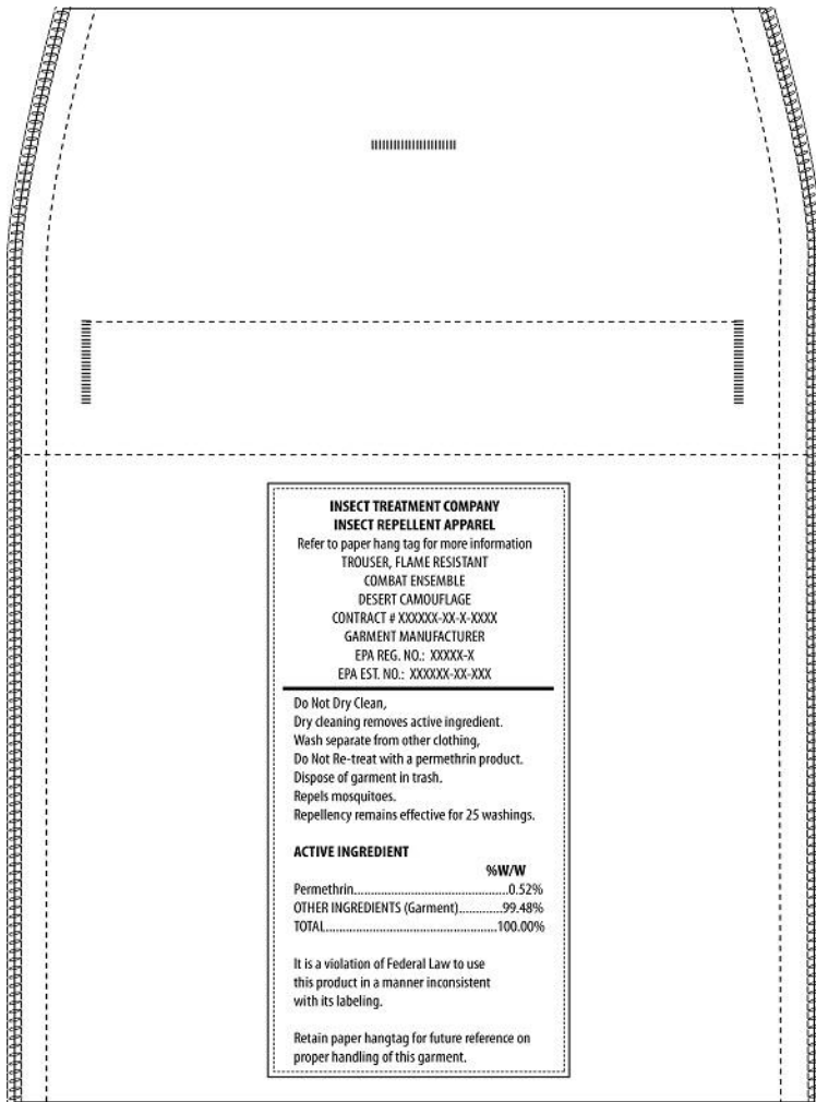
Figure 6, InsectProtection/Brand Label Placement – Right Rear Pocket Bag
